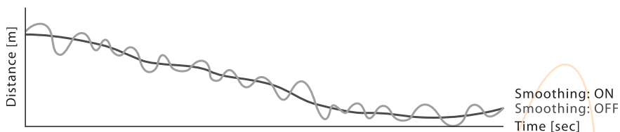
Figure 16 :: Data smoothing
